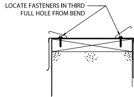
ANCHOR CLIP FASTENING-DETAIL A
