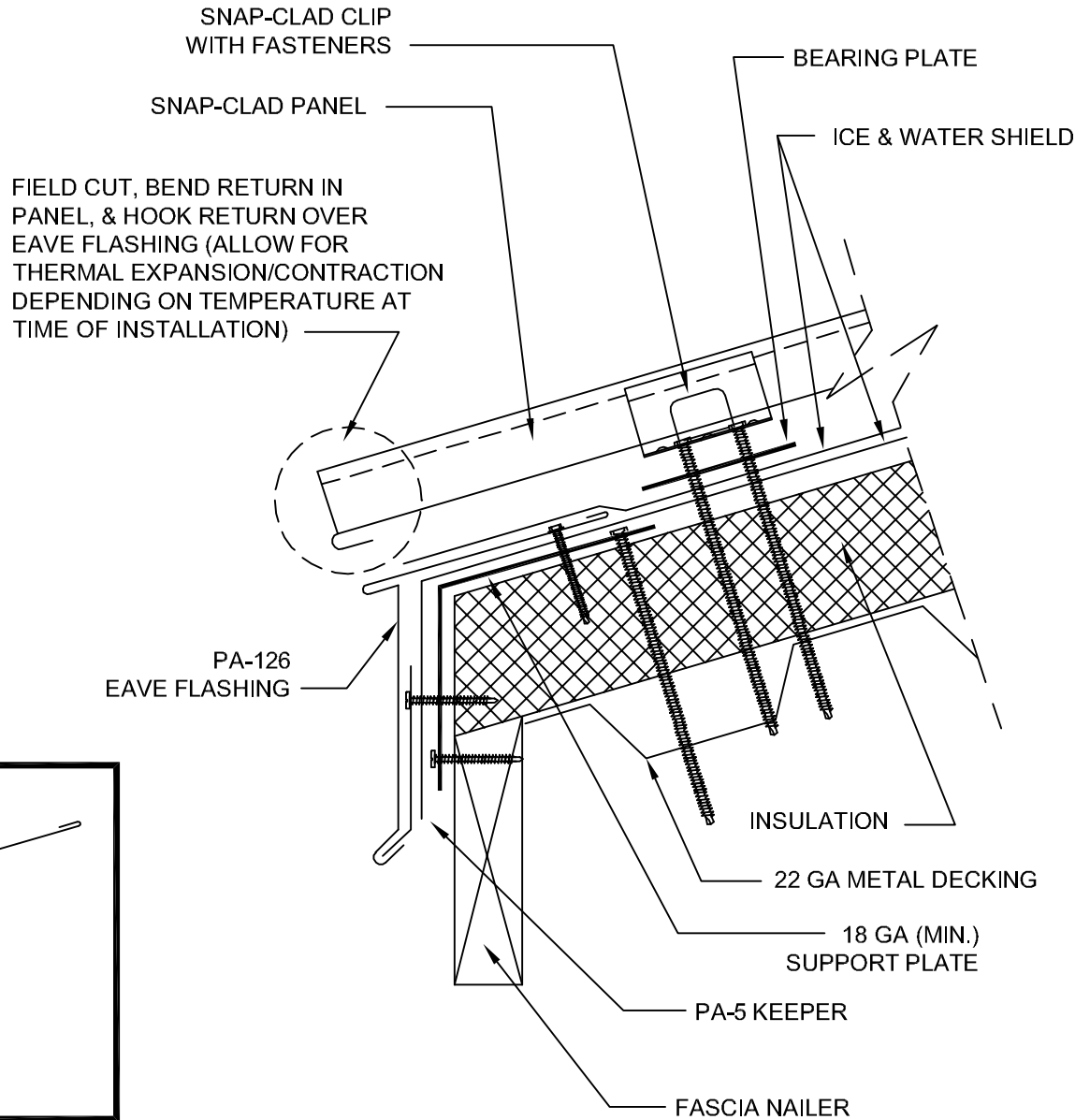
FLASHING COMPONENTS
