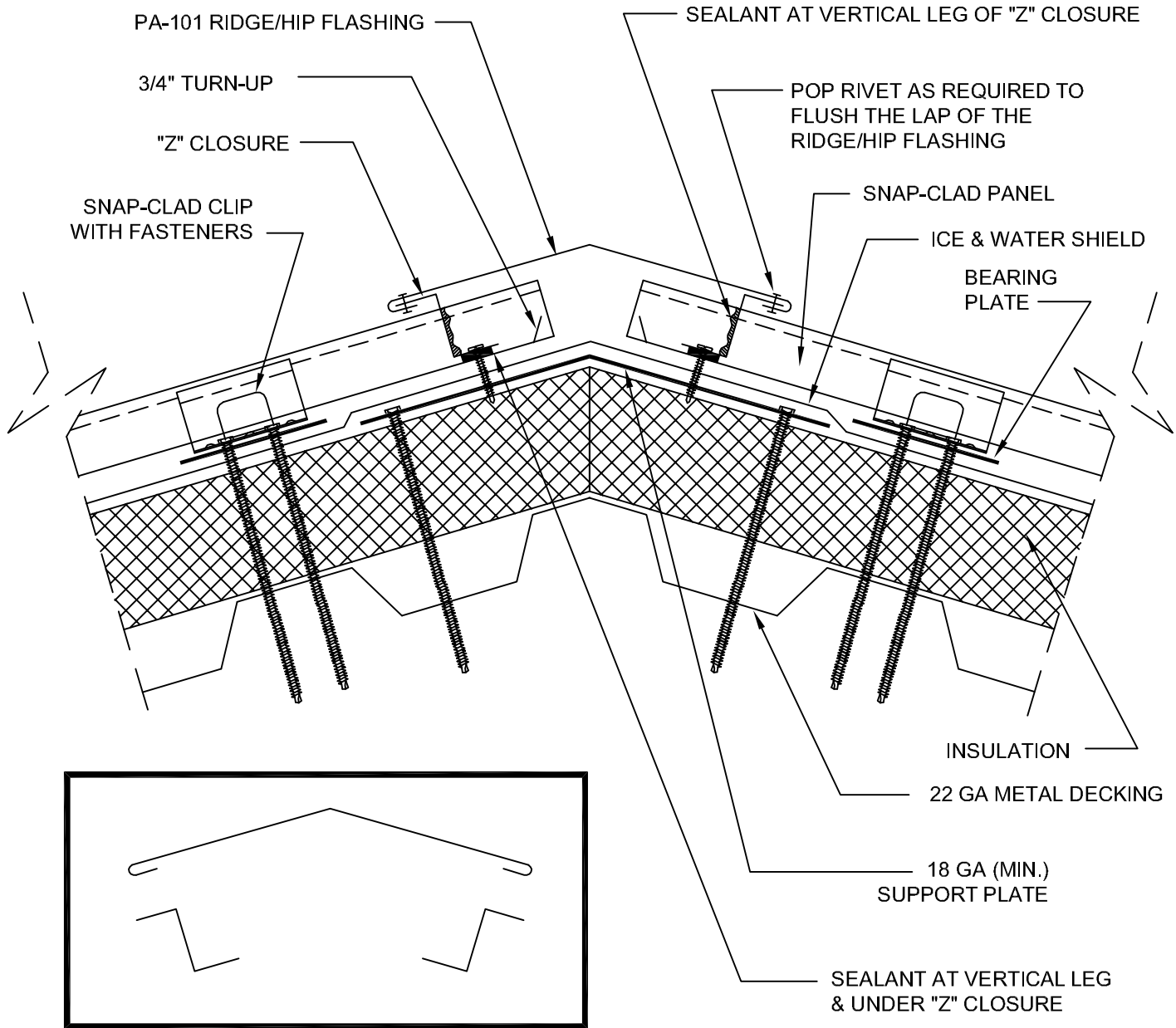
FLASHING COMPONENTS
