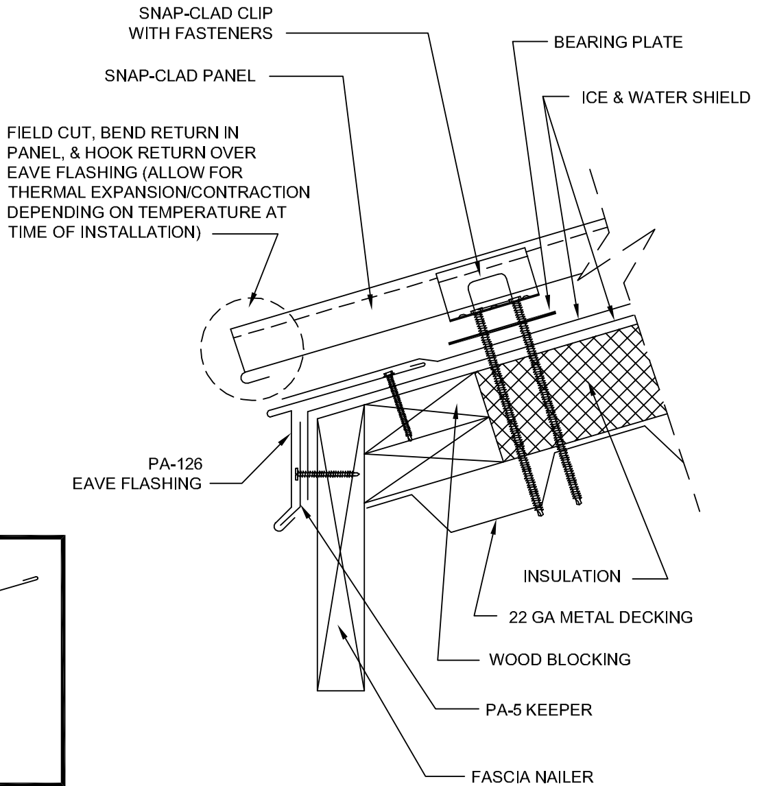
FLASHING COMPONENTS
