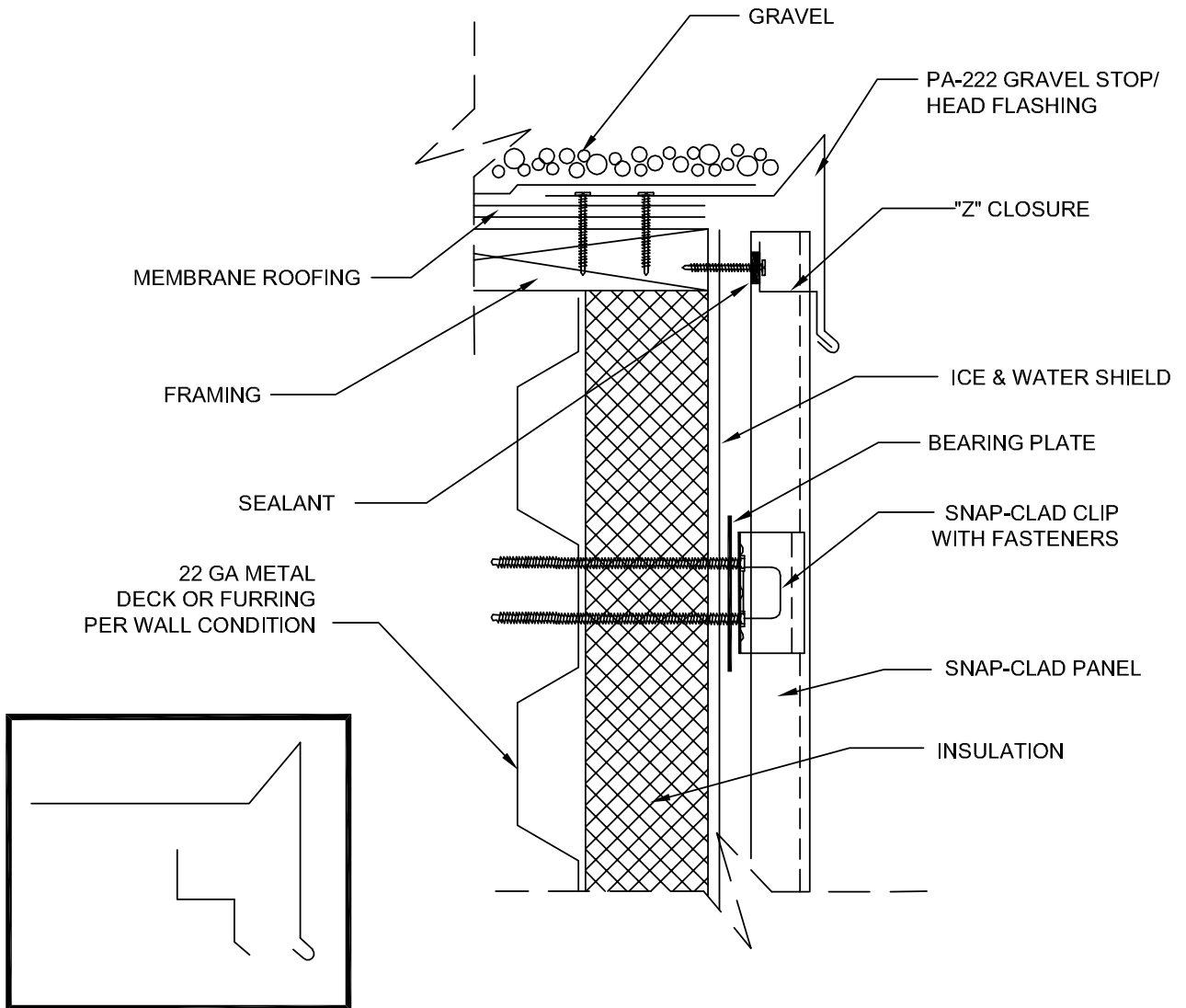
FLASHING COMPONENTS
