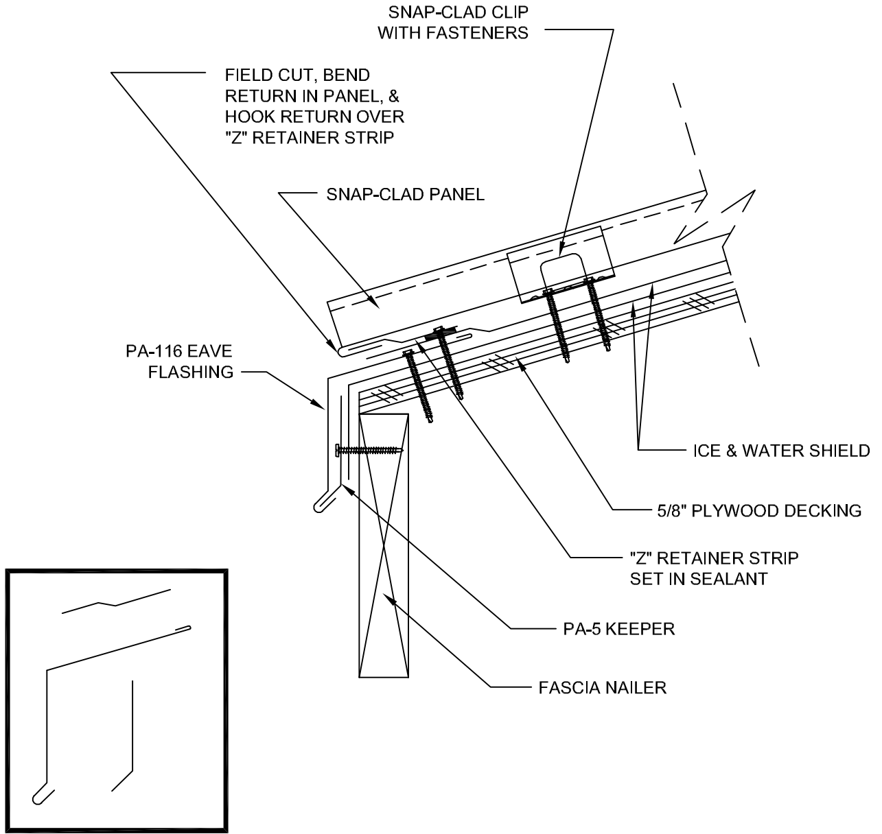
FLASHING COMPONENTS
