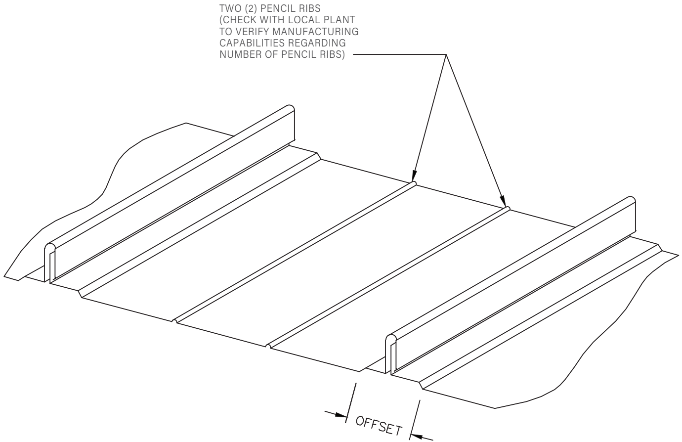
REDI-ROOF PANEL WITH OFFSETS AND PENCIL RIBS ISOMETRIC VIEW
