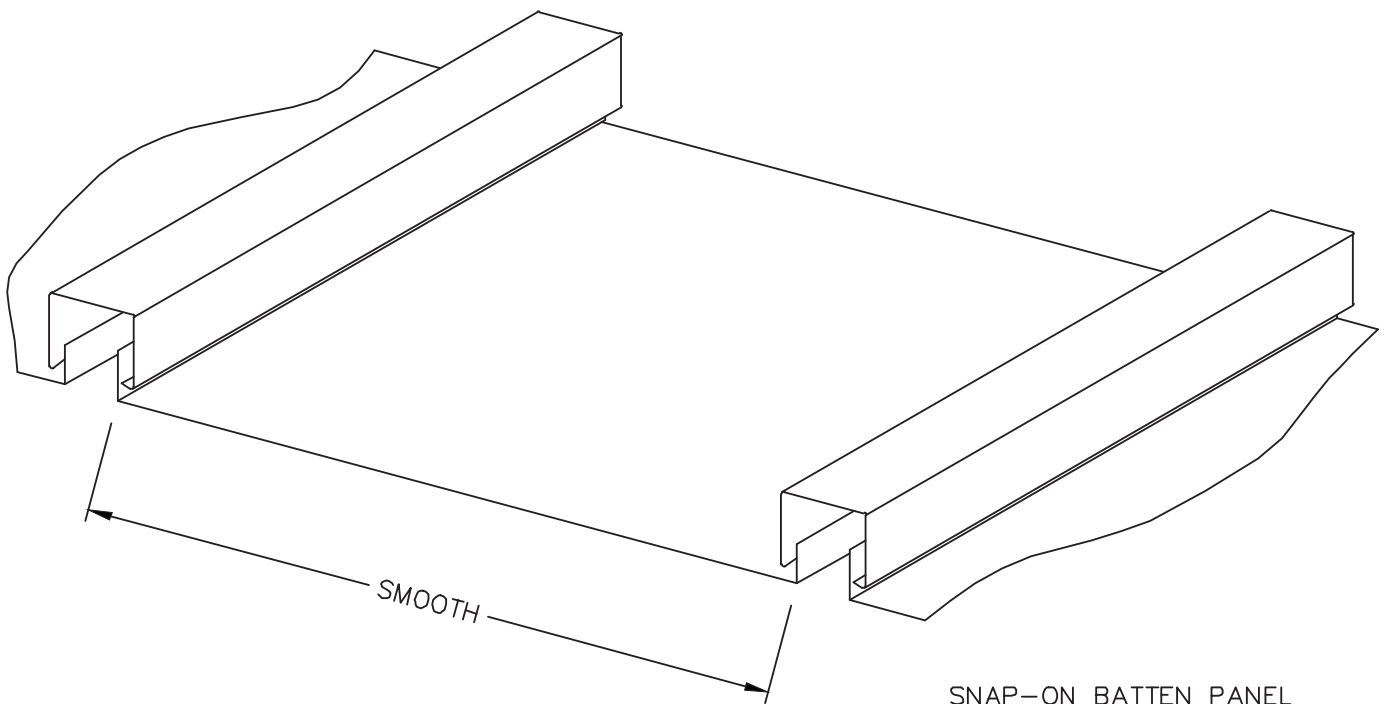
SNAP-ON BATTEN PANEL SMOOTH ISOMETRIC VIEW
