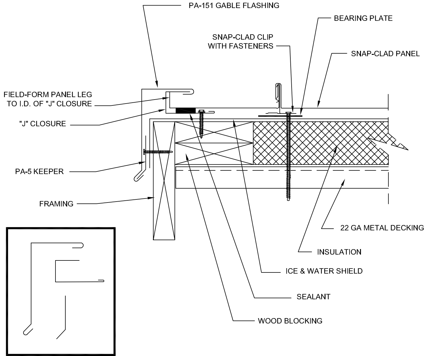
FLASHING COMPONENTS
