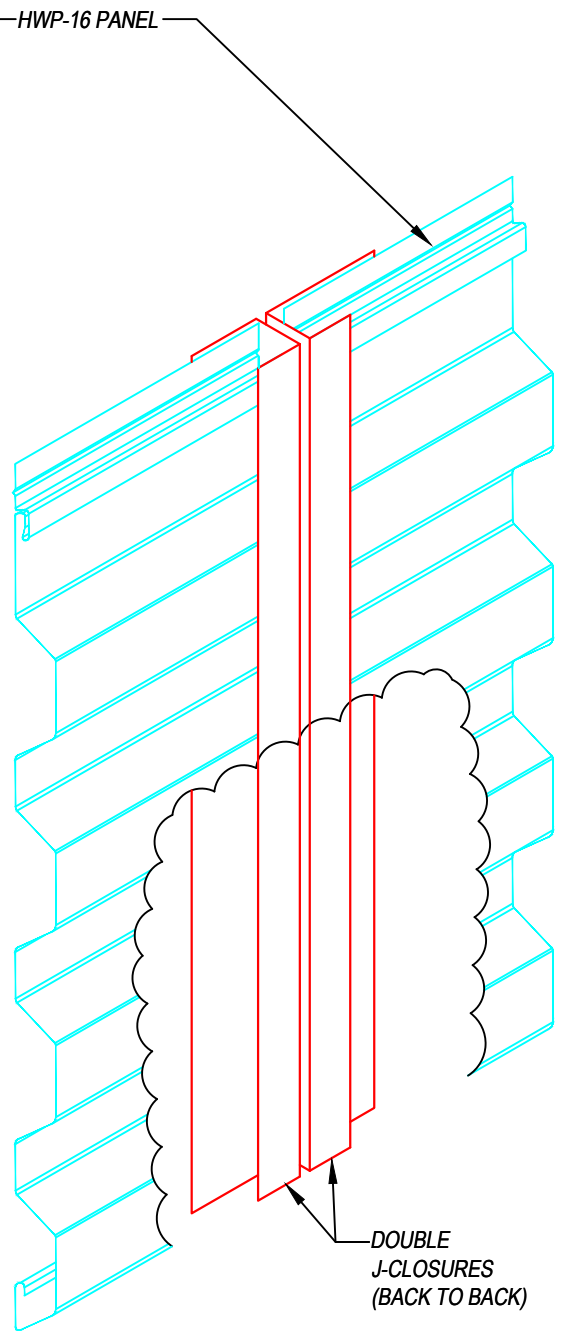
WALL SPLICE OPTION #2
