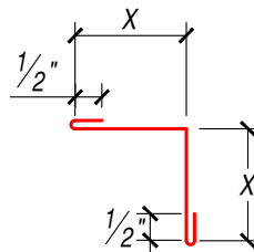
INSIDE CORNER
