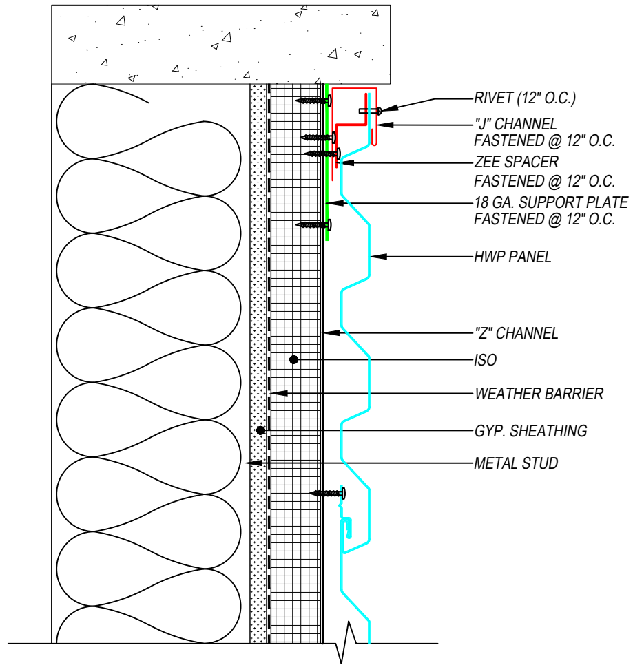
SECTION VIEW
