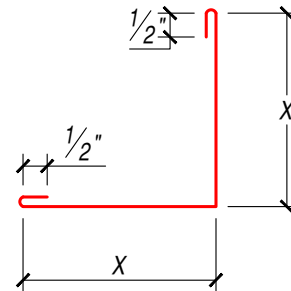
OUTSIDE CORNER
