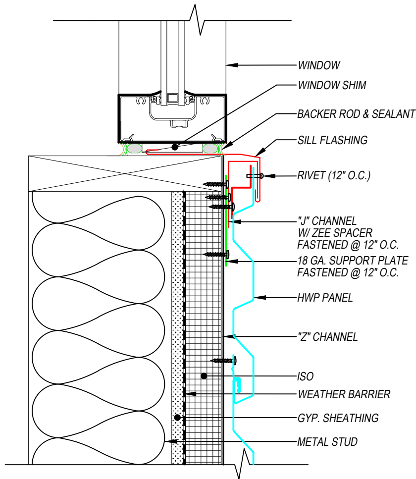
SECTION VIEW
