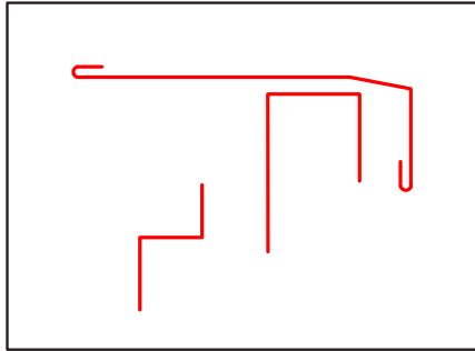
FLASHING COMPONENTS
