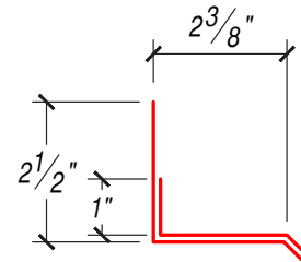
SILL
