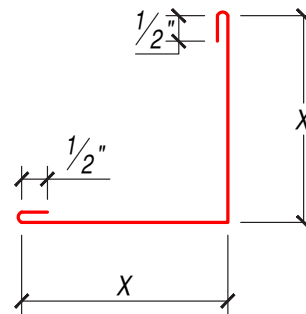
OUTSIDE CORNER
