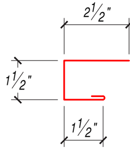
J-CHANNEL
