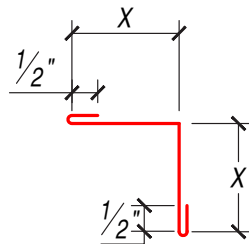
INSIDE CORNER
