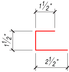
J-CHANNEL
