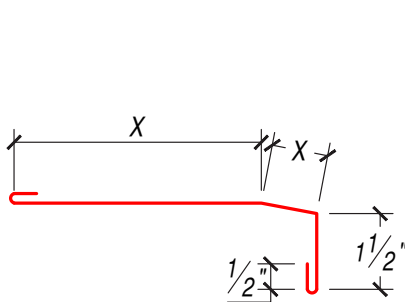
HEAD FLASHING @ WINDOW SILL
