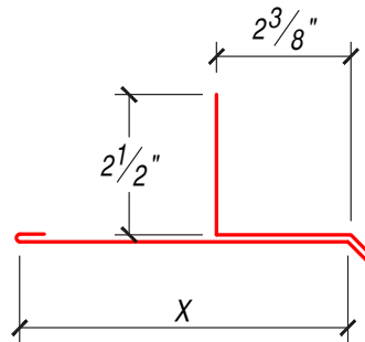
SILL FLASHING @ WINDOW HEAD
