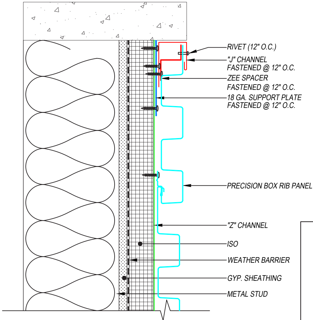
SECTION VIEW
