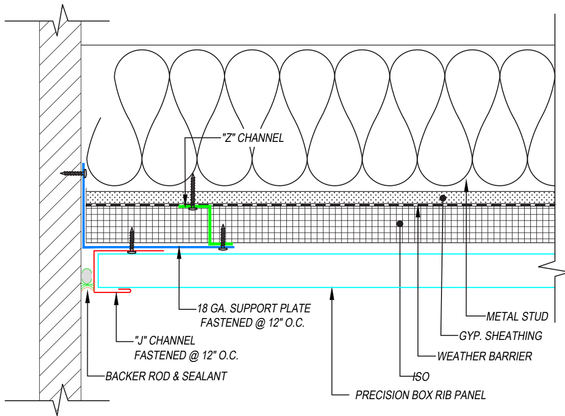
FLASHING COMPONENTS
