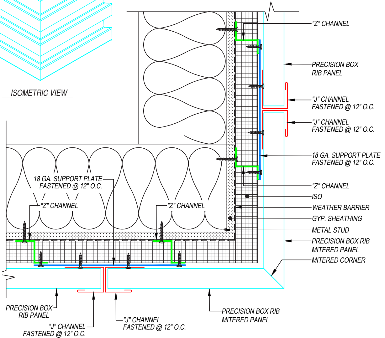
PLAN VIEW
