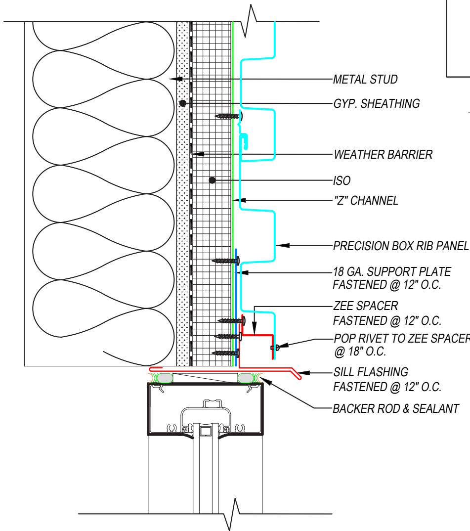
SECTION VIEW
