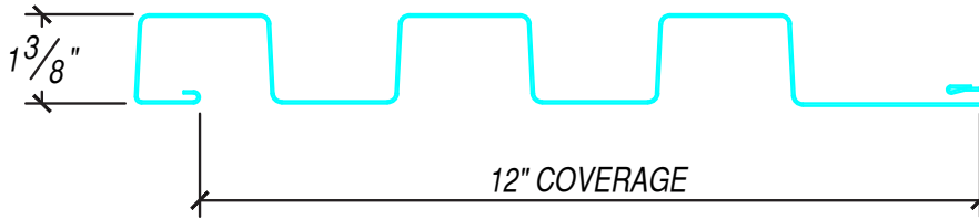
PRECISION SERIES BOX RIB (CLIP OPTION)
