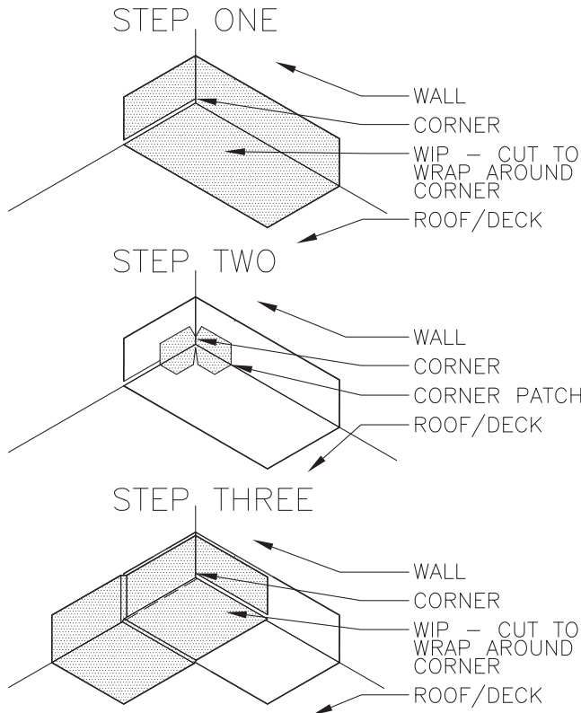
INSIDE CORNER FLASHING
