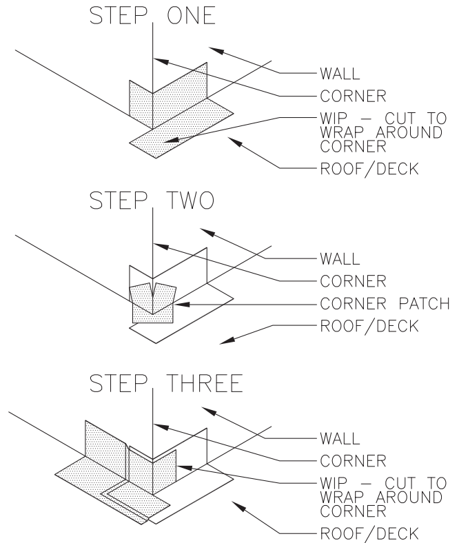
OUTSIDE CORNER FLASHING
