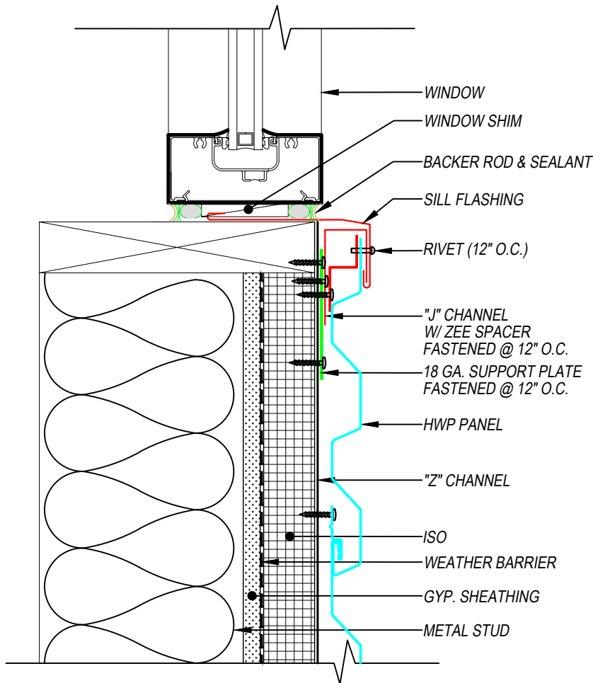
SECTION VIEW
