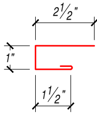
J-CHANNEL
