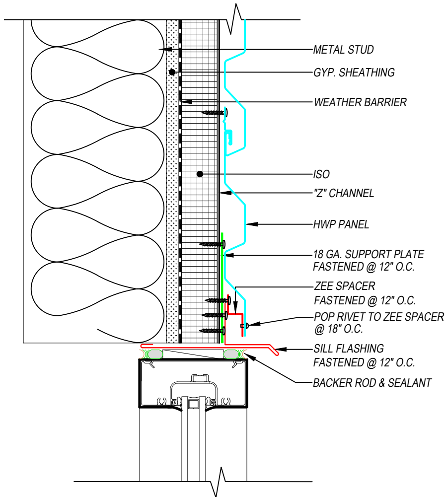
SECTION VIEW
