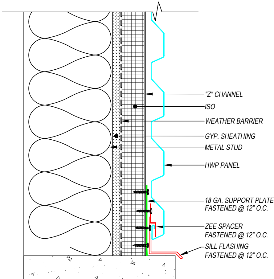
SECTION VIEW
