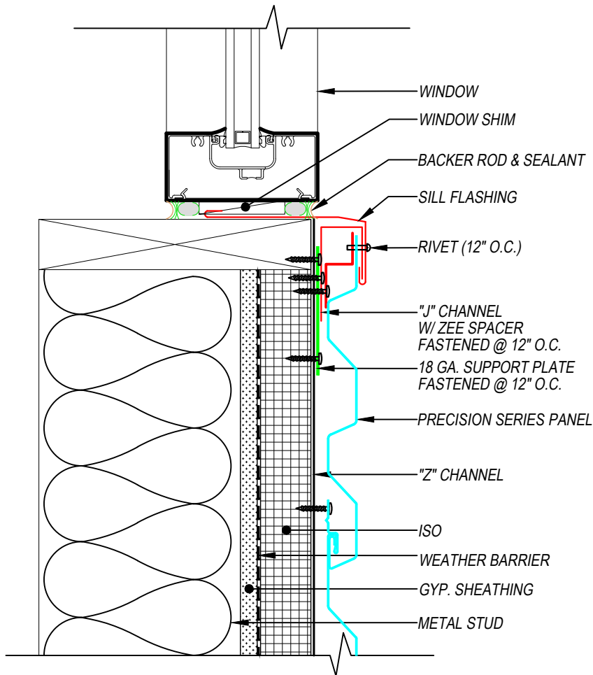
SECTION VIEW
