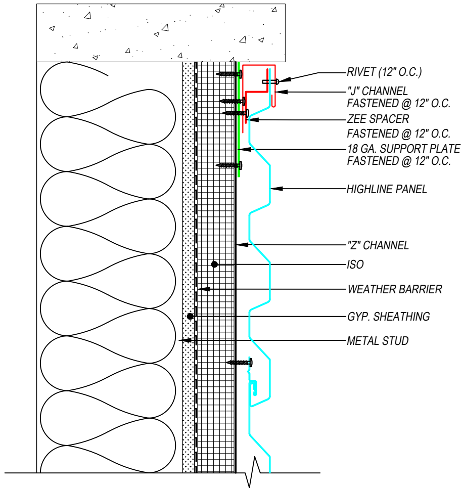
SECTION VIEW
