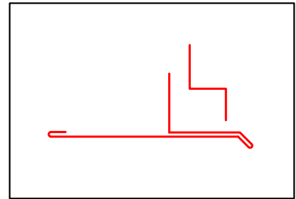
FLASHING COMPONENTS
