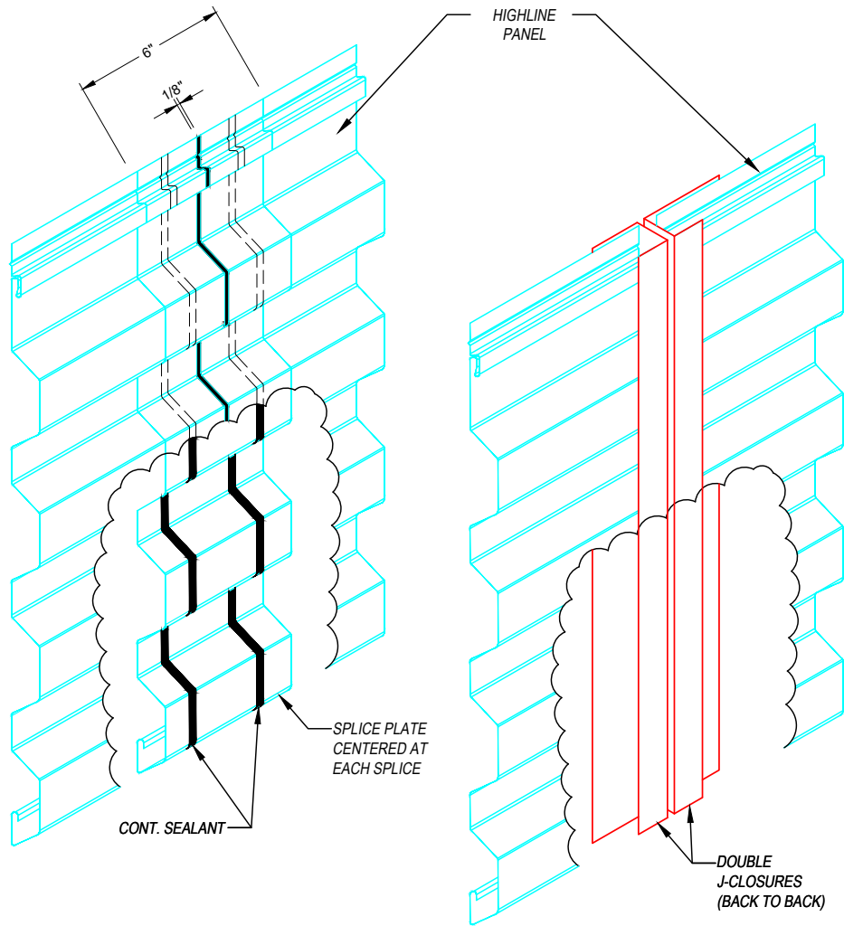
WALL SPLICE OPTION #1
