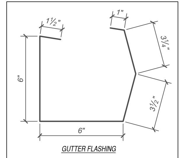
FLASHINGS
