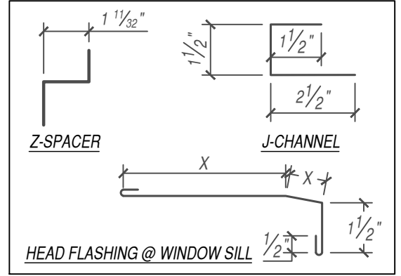
FLASHINGS
