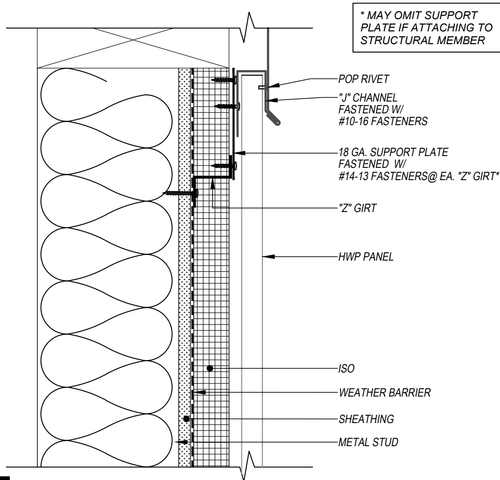
CONCEALED CLIP END
