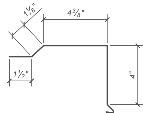
GABLE FLASHING
