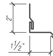
SILL @ WINDOW HEAD
