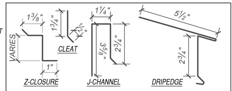
FLASHINGS
