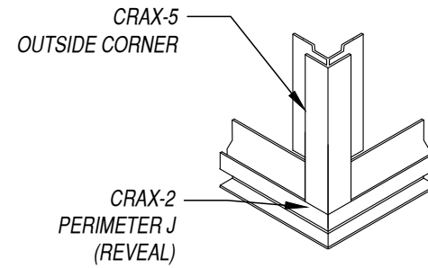
12B BASE OUTSIDE CORNER, OPTION 2
