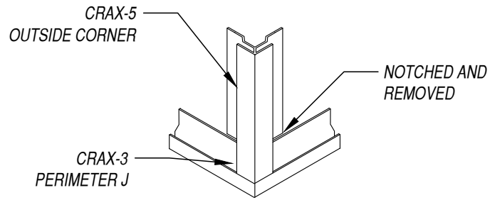
12A BASE OUTSIDE CORNER, OPTION 1
