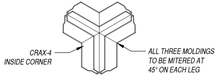
17 THREE WAY CORNER
