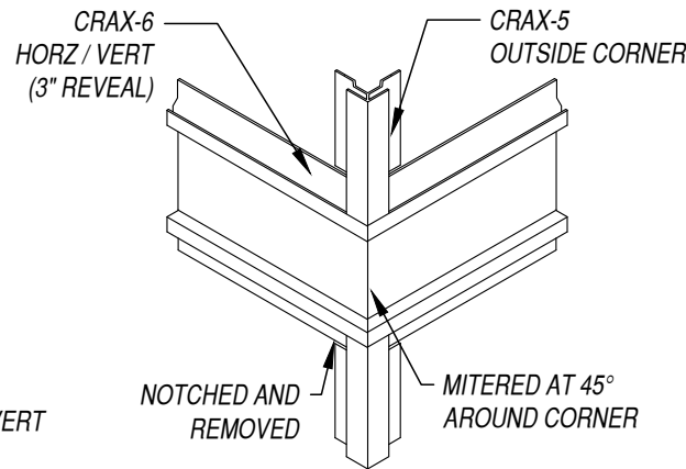
19D OUTSIDE CORNER OPTION 4
