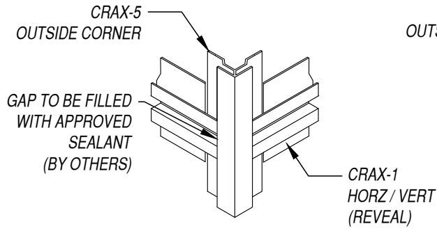
19A OUTSIDE CORNER OPTION 1
