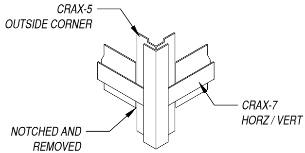
19B OUTSIDE CORNER OPTION 2
