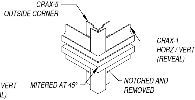
19C OUTSIDE CORNER OPTION 3
