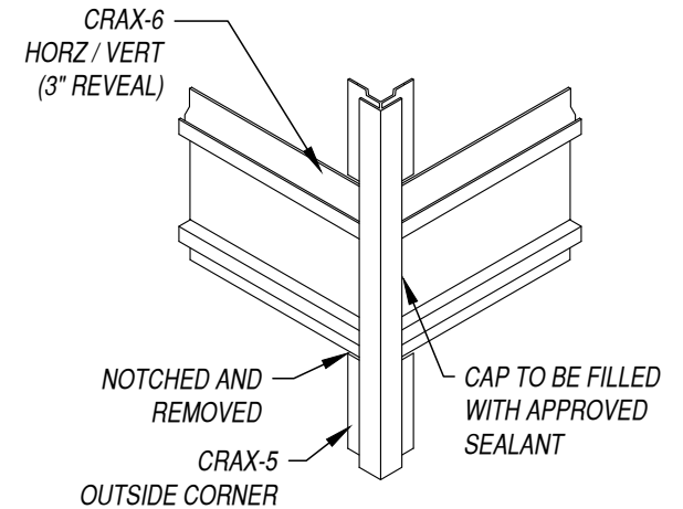
19E OUTSIDE CORNER OPTION 5
