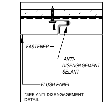
FLUSH ANTI-DISENGAGEMENT OPTION
